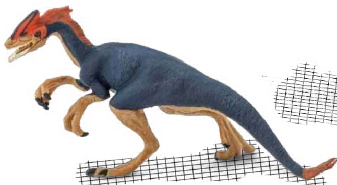
Guanlong (Goo-ON-long)
