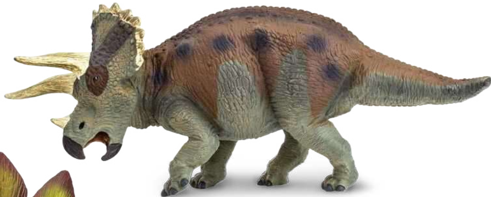
■ Triceratops (try-SER-a-tops)
