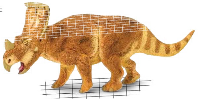
■ Vagaceratops (vag-a-SER-uh-tops)
