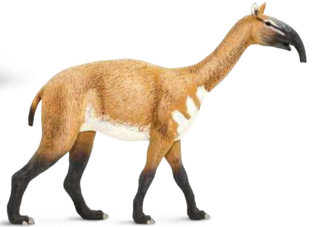
■ Macrauchenia (MACK-row-KEEN-yuh)
