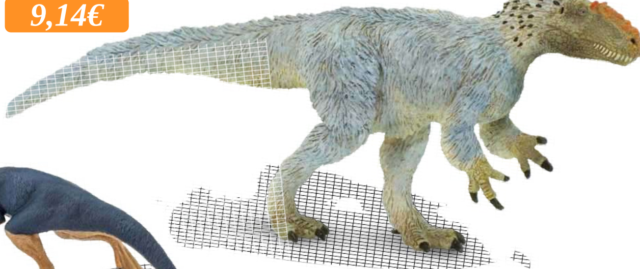
Yutyrannus (you-tih-RAN-us)
